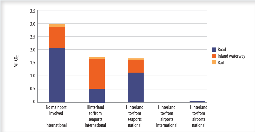
Figure 10 CO 2 emissions of international freight transport per mode and territory (Mt in 2015).
