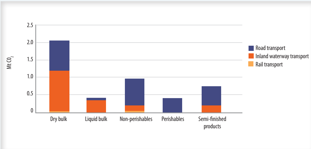
Figure 12 CO 2 emissions per segment of port-related hinterland and continental freight on Dutch territory (Mt in 2015).
